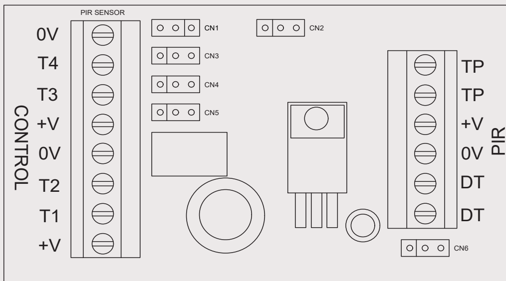
Figure 1 – Control PCB Outline
