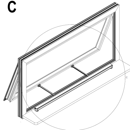
C: Top hung outward opening
